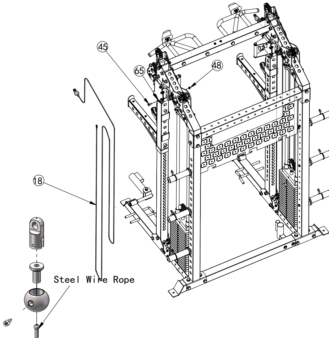
Disassembly and Assembly Schematic Diagram of the Steel Wire Rope Ball Head
